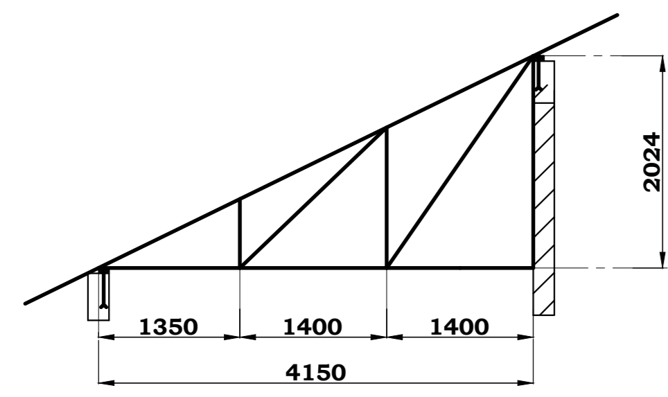
TYPICAL TRUSS 3 -6No. ALL MEMBERS - 100x50mm TIMBER SCALE 1:50
