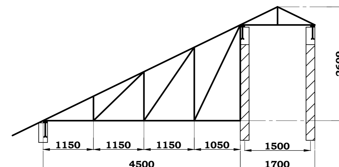
TYPICAL TRUSS 2 -3No. ALL MEMBERS - 100x50mm TIMBER SCALE 1:50
