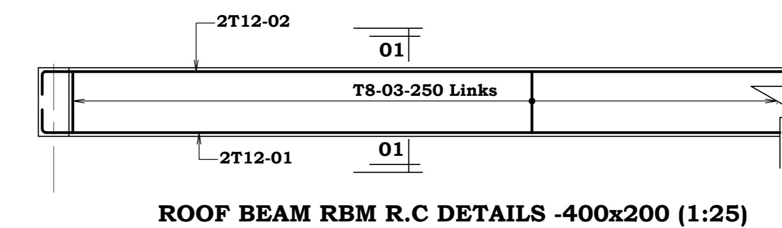
ROOF BEAM RBM R.C DETAILS -400x200 (1:25)
