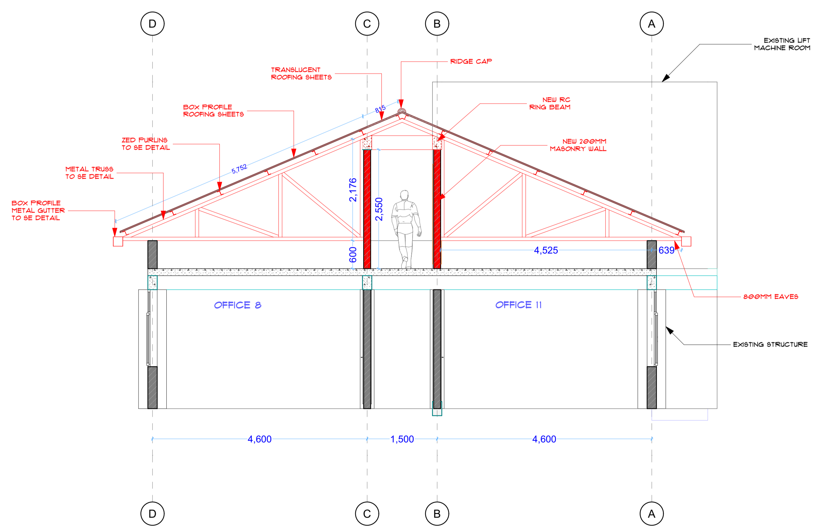
Building Section (1)
