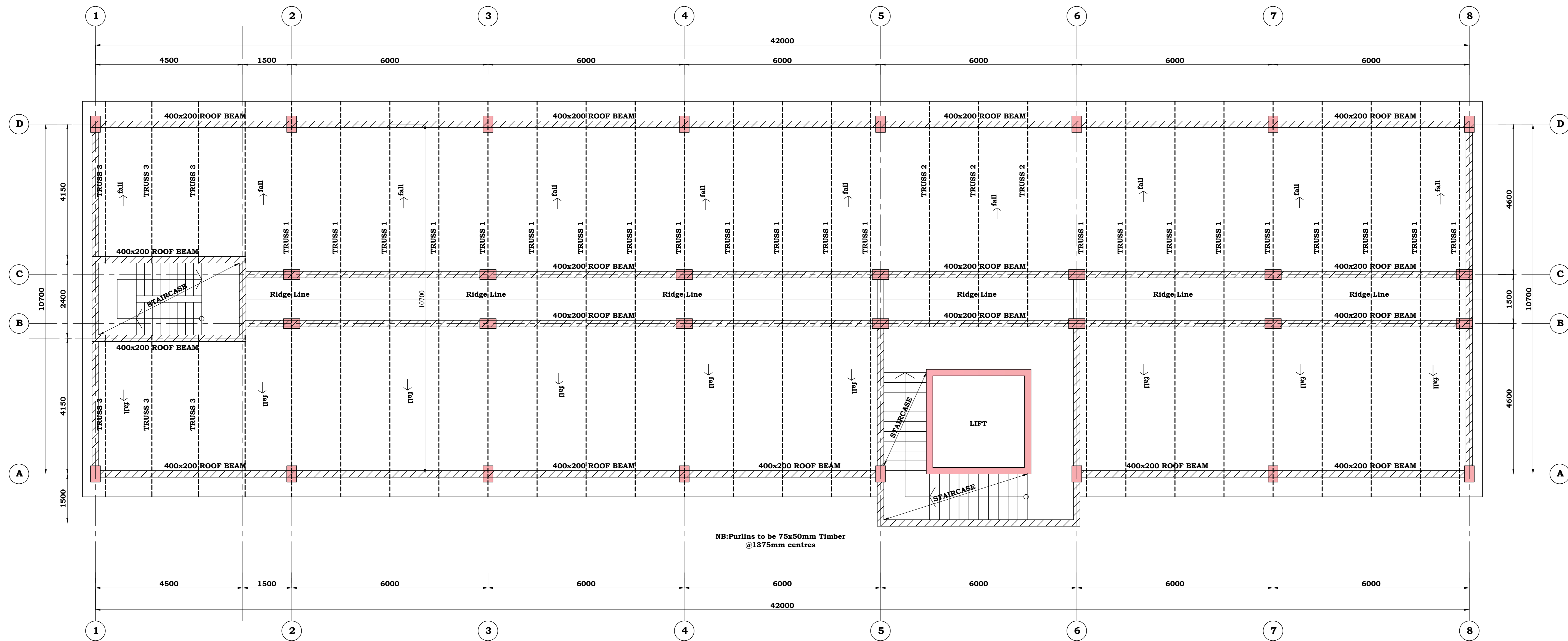
ROOF LAYOUT PLAN AND DETAILS - (SCALE 1:50)
