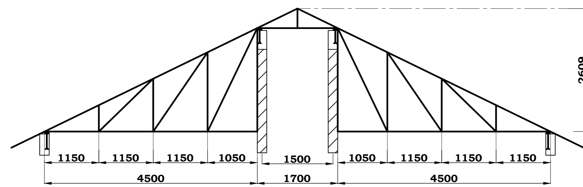
TYPICAL TRUSS 1 -22No. ALL MEMBERS - 100x50mm TIMBER SCALE 1:50
