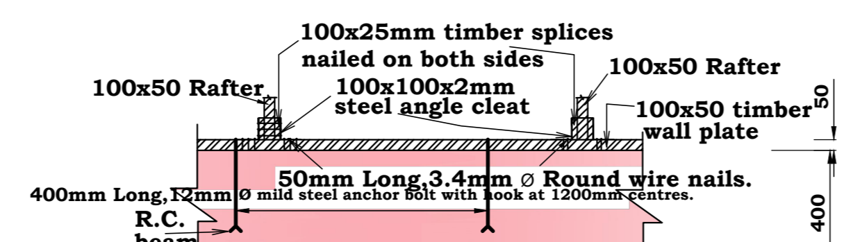
TYPICAL TRUSS ANCHORAGE DETAILS SCALE 1:25
