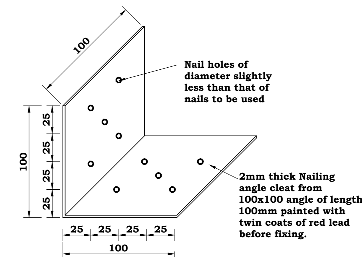
DETAIL OF NAILING ANGLE CLEAT 1:2
