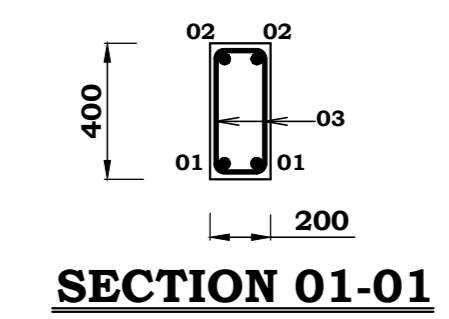
SECTION 01-01
